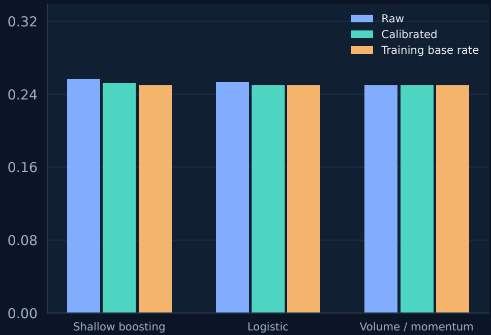
Probability error · Brier, lower is better
