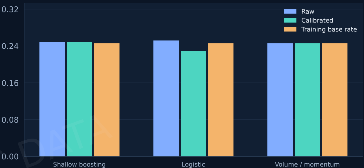
Probability error · Brier, lower is better
