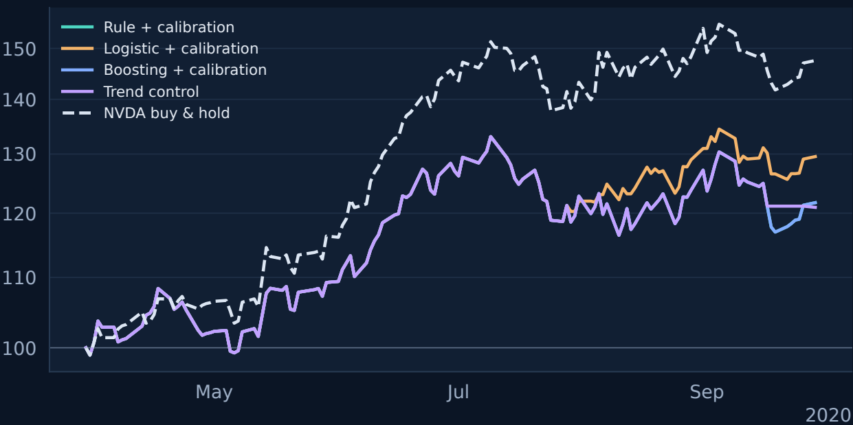
Net wealth · initial = 100 · log scale
