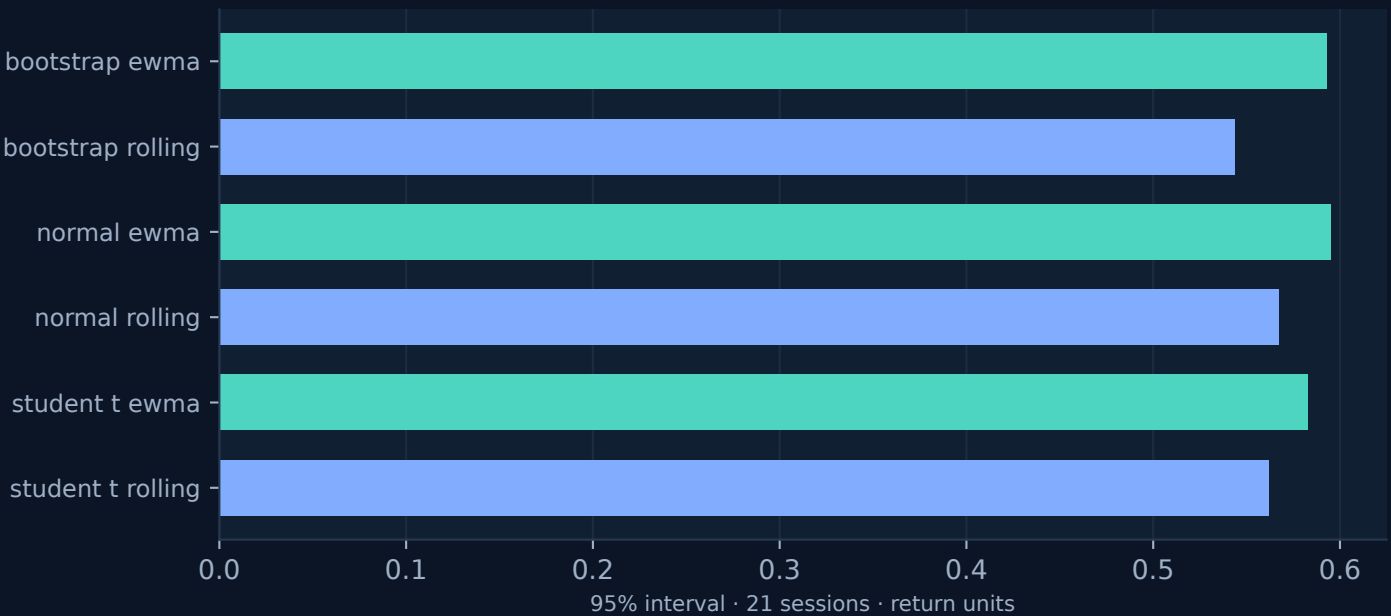
Interval score · lower is better
