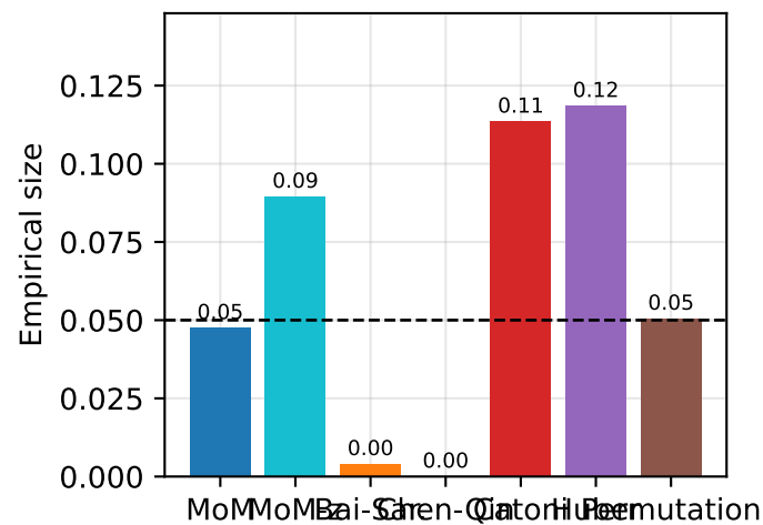
Contaminated noise
