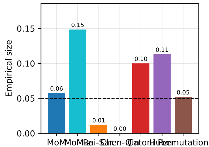
Contaminated noise
