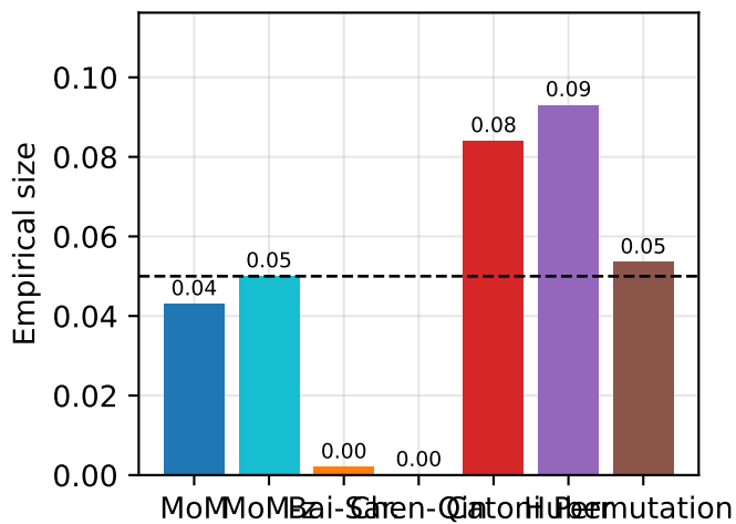
Log-normal noise
