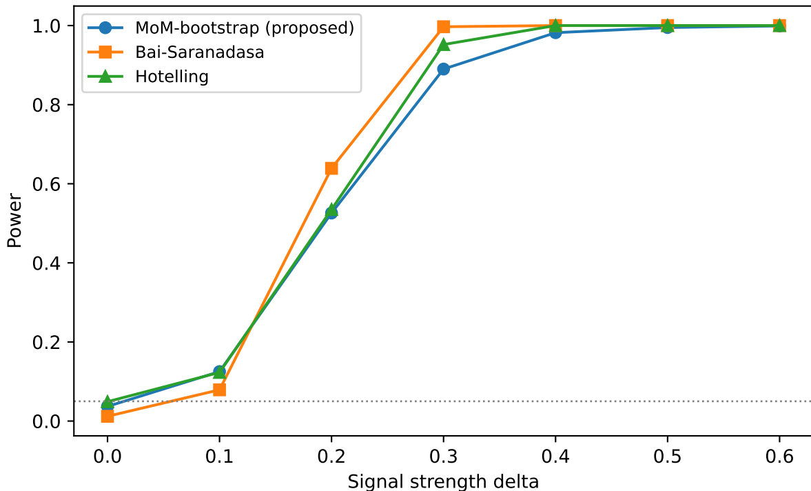
Power vs signal (Gaussian, p=100 , n=200 )
