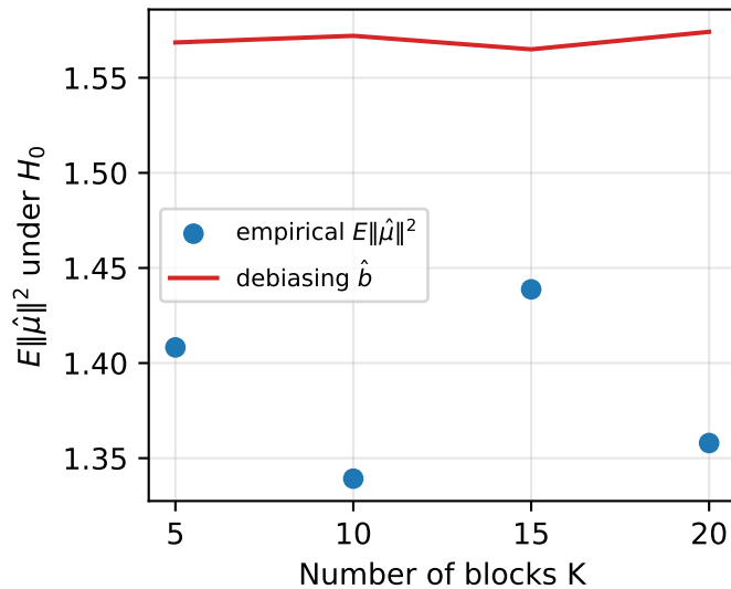
t(5) noise
