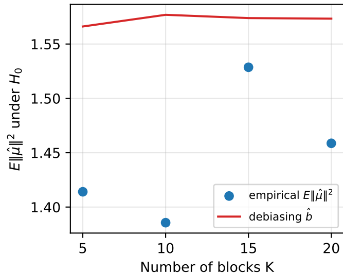
Gaussian noise
