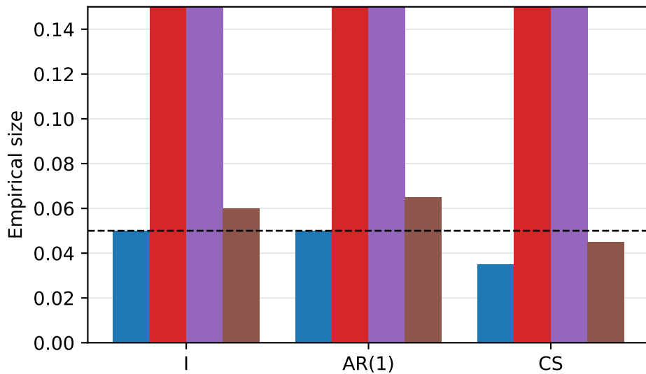
Gaussian, p=500 , n=100
