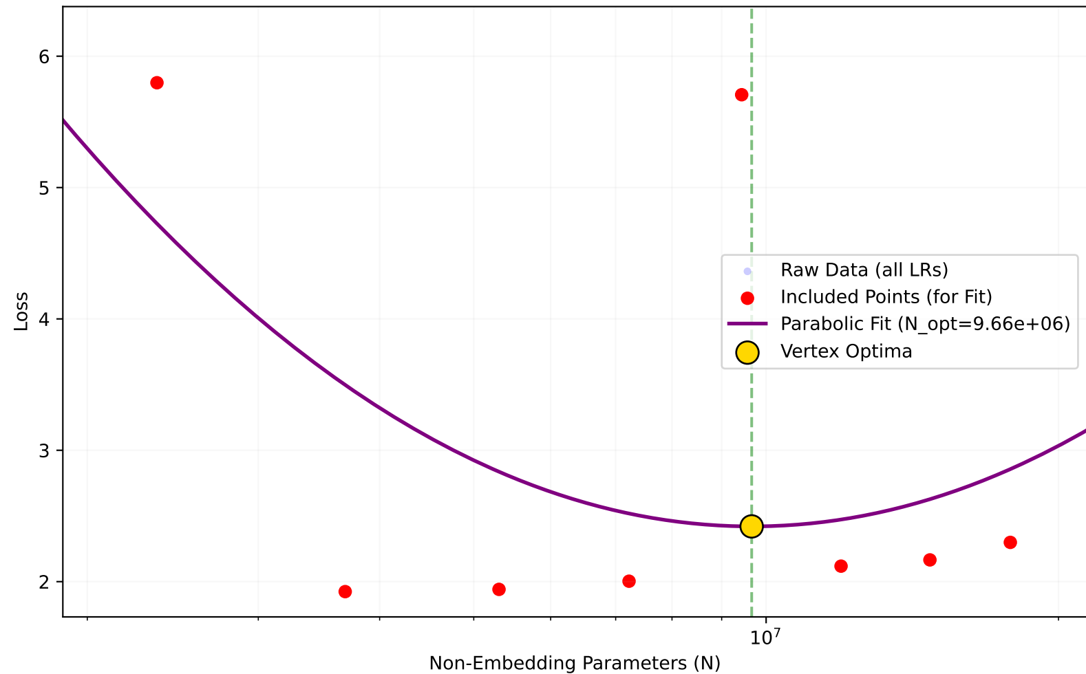
Iso-FLOPs Profile
