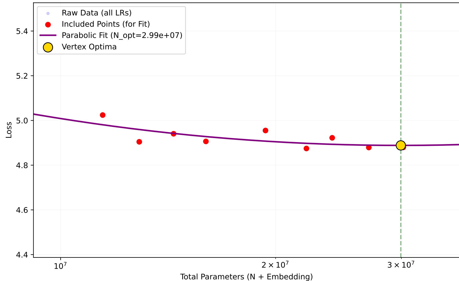
Iso-FLOPs Profile
