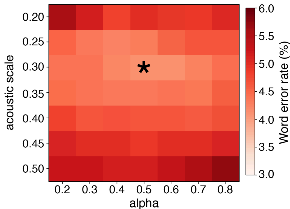
Figure S10: Offline language model parameter sweeps informed subsequent online parameter choices.
