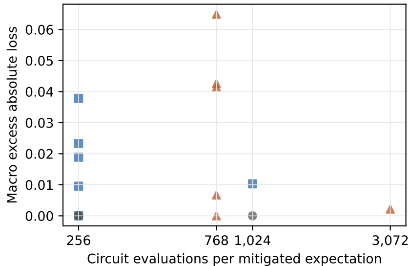
Harm-cost frontier
