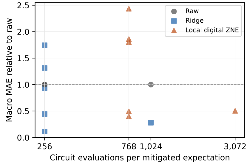
Accuracy-cost frontier
