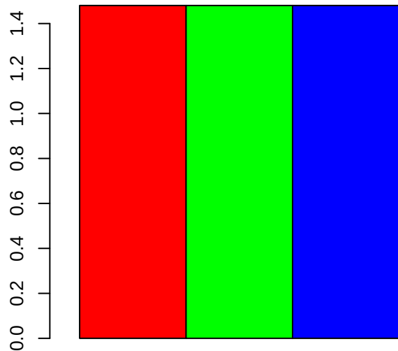
Residual variance
