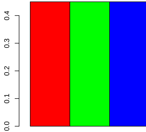
Genetic variance
