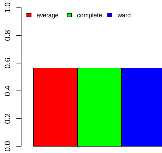
Heritability
