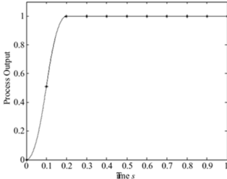
Fig. 5.14 Step response
