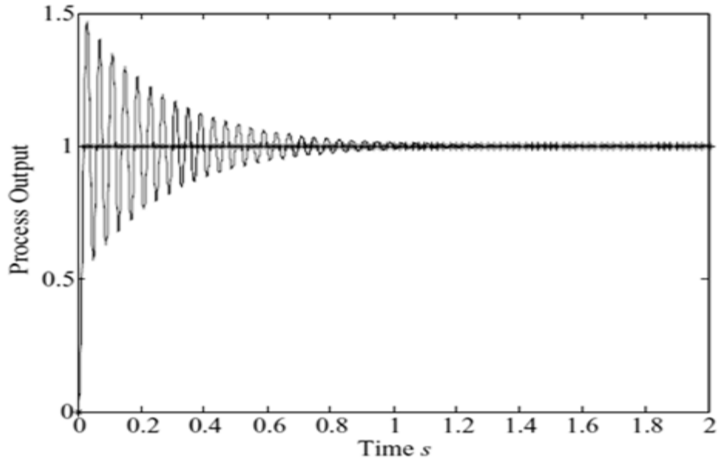
Figure 5.10 Step response
