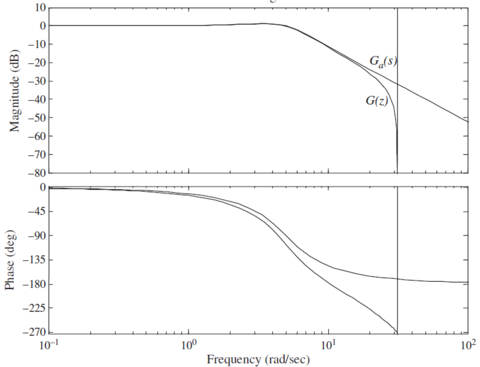
Bode Diagram
