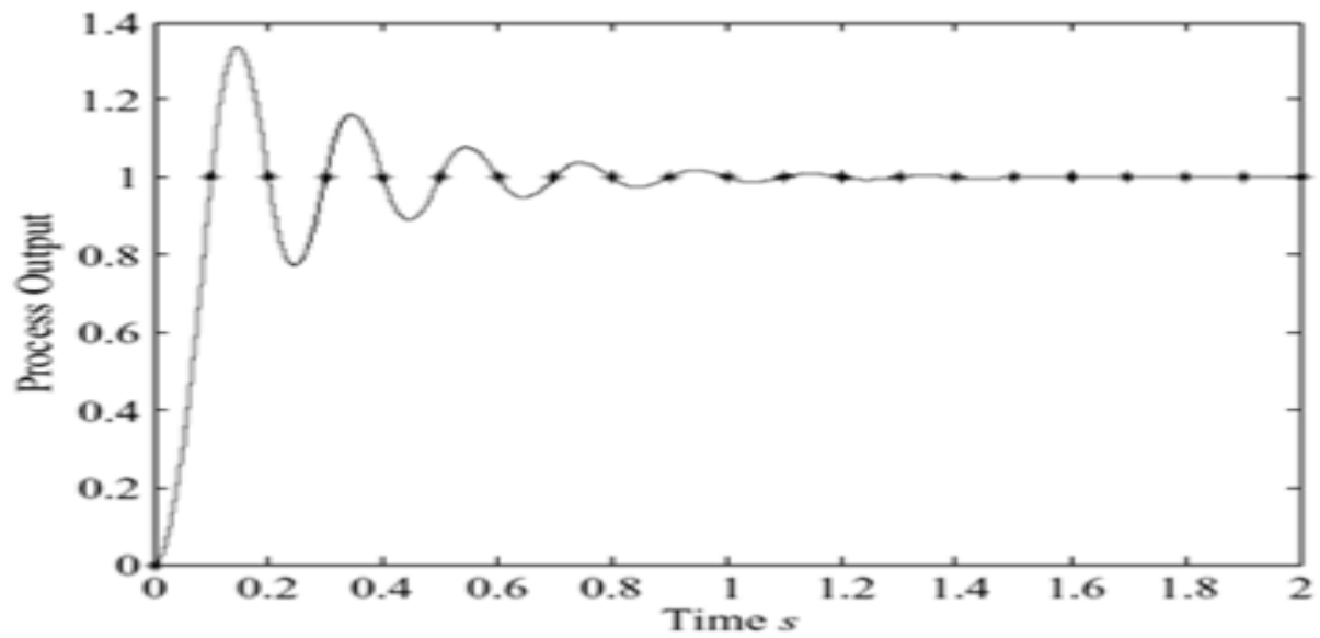
Figure 5.12 Step response
