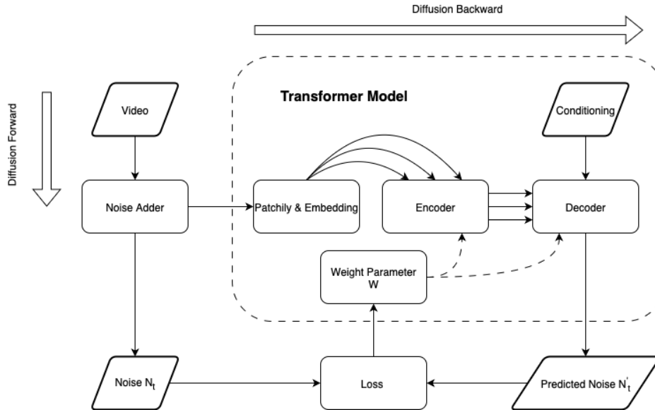
Figure 1: Frame of Video Generation Model
