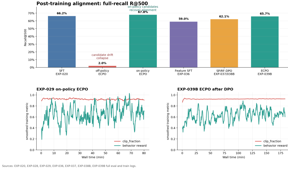
Figure 4: Post-training alignment curves and collapse/recovery behavior.
