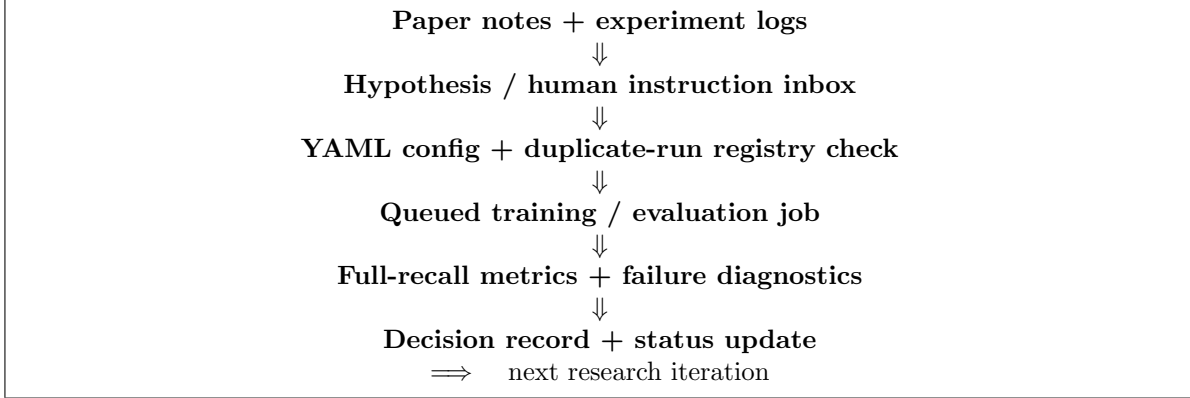
Figure 1: Agentic research loop implemented by NANOGENREC. The loop turns paper reading, experiment design, execution, evaluation, and decision logging into auditable repository state.
