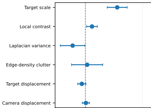
Faster R-CNN
