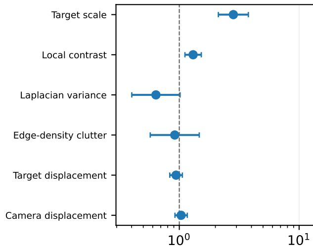
RT-DETR-L
