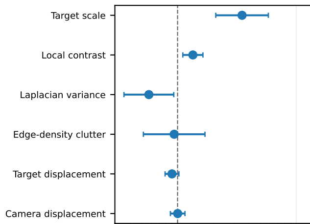
RetinaNet
