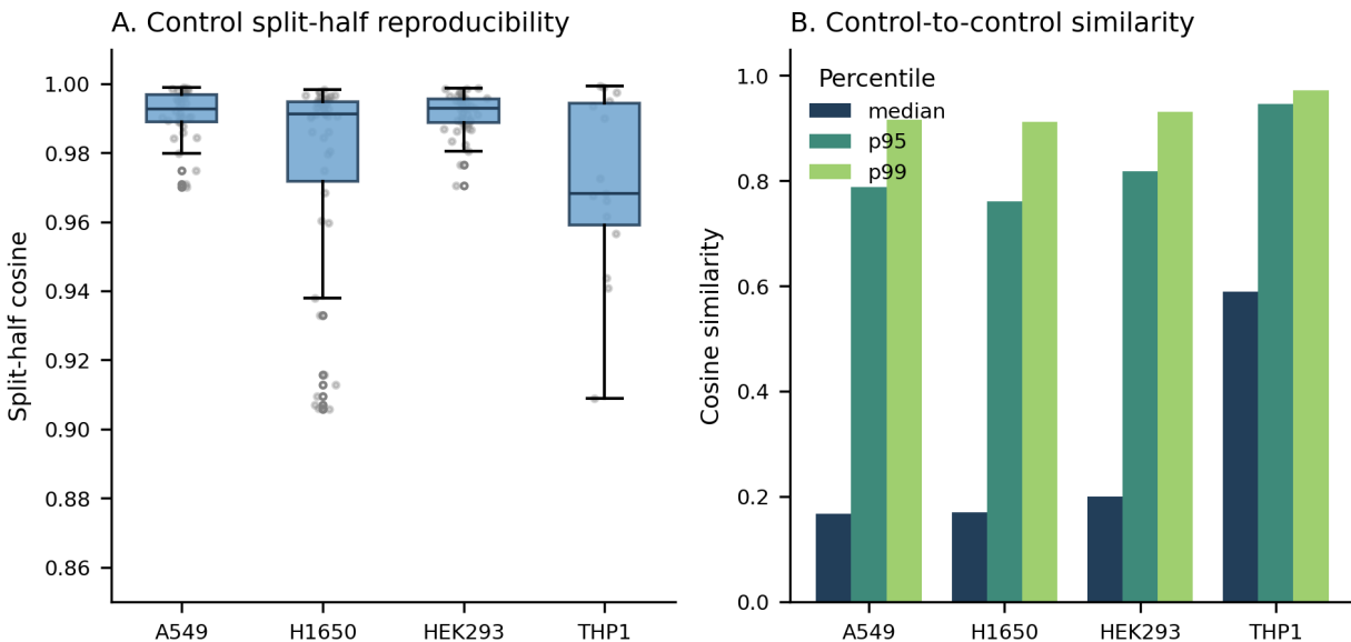
Figure 1: Figure 1. Named controls show high split-half reproducibility across all four cell lines, establishing a strong assay floor for downstream chemistry-to-phenotype modeling.
