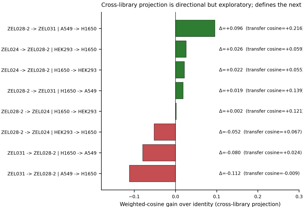
Figure 5: Figure 5. Cross-library projection results. Some cross-library projections are positive, but performance remains small, asymmetric, and sensitive to which library acts as teacher. The result is best read as a design brief for a prospective cross-library dataset.
