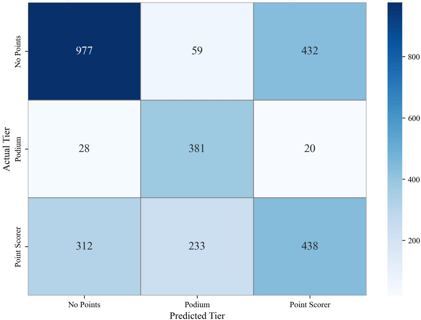
Figure 4: Confusion Matrix — LOGO-CV (Accuracy: 62.36%)
