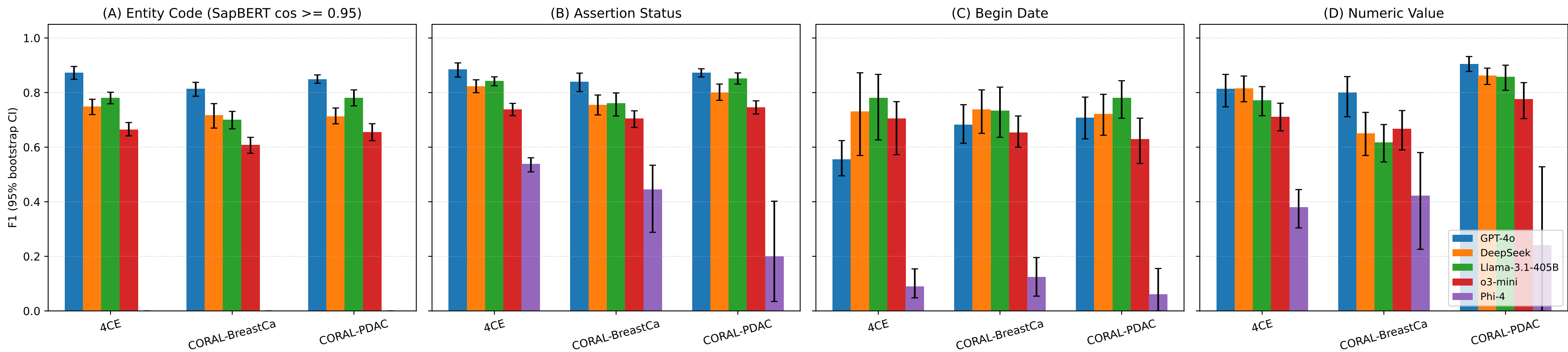
Figure 3A-D: F1 with 95% bootstrap CIs (n_boot=2000, seed=20260525)
