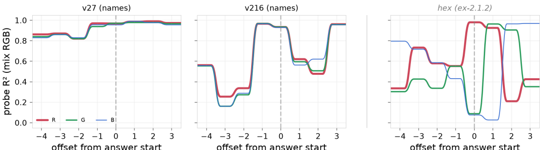
The answer-emission schedule at the final residual depth (seed 0). Each line is R^2 for one RGB channel across offsets from the first character of the answer; the answer sits at offsets 0–3, and the last characters of the prompt are the negative offsets. Lines are drawn as steps because each offset is a separate character position, with the value held across the position and ramping between; line width tapers R \rightarrow G \rightarrow B so an offset where all three agree reads as nested bands rather than as whichever channel drew last. Hex answers (right, from the ex-2.1.2 base-grammar conditions) spell one channel per digit, and the probe found each channel computed just in time and dropped once emitted. Opaque names cannot be written that way, and H4 predicts all three channels stay decodable across the window.
