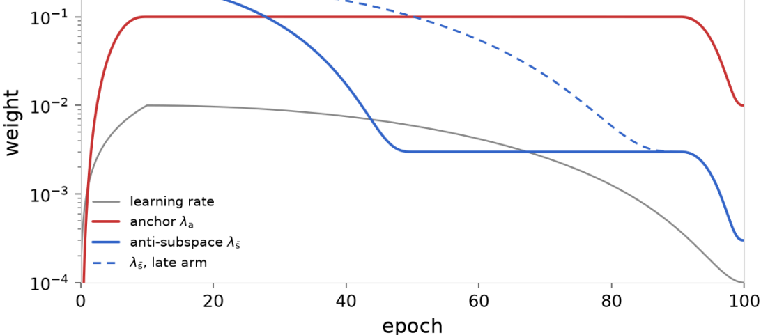
The three schedules at the scoring rung ( \lambda_a = 0.1 ), log scale. The anti-subspace term opens at 2.5\lambda_a dominant before the anchor arrives, and anneals to 0.03\lambda_a by epoch 50 (the M1/ex-2.9.1 keyframes, mapped by fraction of training). The dashed line is the span-anti-late arm, which reaches the hold ratio at epoch 90 instead. From epoch 90 the anchor and anti-subspace weights share the end-of-training anneal to a floor of 0.1\times their held values.
