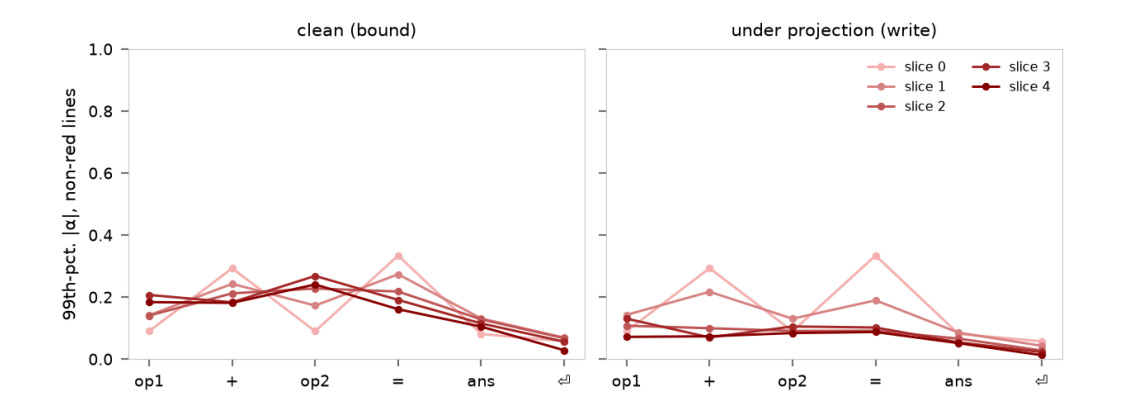
The bound and the write under projection ,fallback condition. The 99th-percentile alignment over the non-red lines at each (slice, position), seed mean, on the shared 0–1 scale. Left, the clean map, whose arcsine is the bound; right, the alignment arriving at the operator under projection , whose arcsine is the write. Slices run from the embedding (lightest) to the last block (darkest). A deeper line above its clean value would mean a block re-writes the axis after it was removed upstream, which is what a wider edit looks like.
