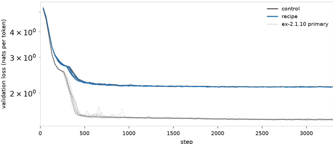
Validation loss over training. Five thin lines per condition on the step axis: the control in grey and the recipe in blue. The ghost lines behind them are the ex-2.1.10 primary (nine seeds) and its control (three), which trained on the one-op grammar at the same step count; their floor sits lower because their corpus held about seventeen copies of each distinct line, where this one holds most lines once. Log scale.
