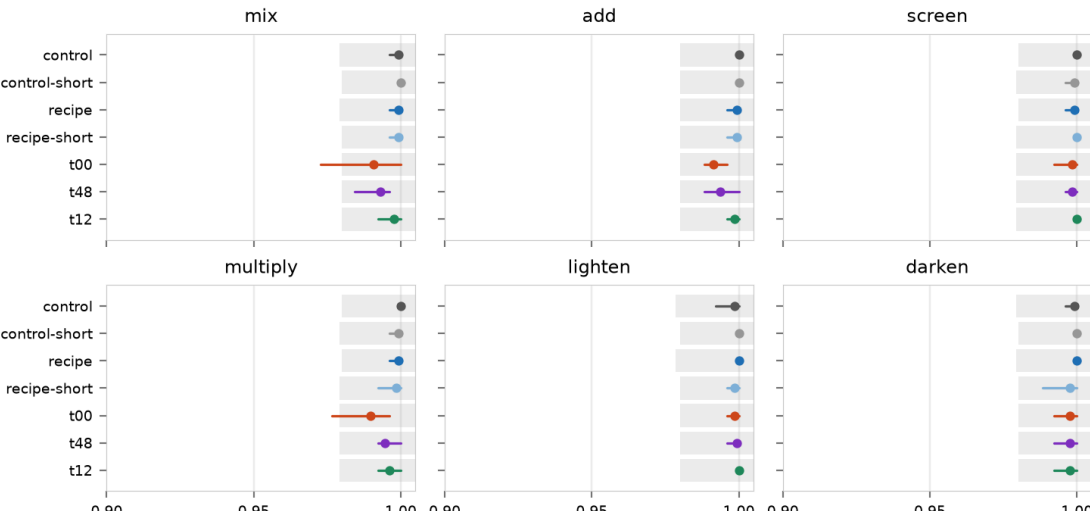
Holdout exact match per op, against the gate. One panel per op; conditions down the side, in their own ink. Each dot is the seed mean, the bar the seed range. The grey strip behind a row is ±0.02 around the seed-mean accuracy of the control of the same length, so a dot outside its strip misses the H1 gate; the two control rows carry their own strips for reference.
