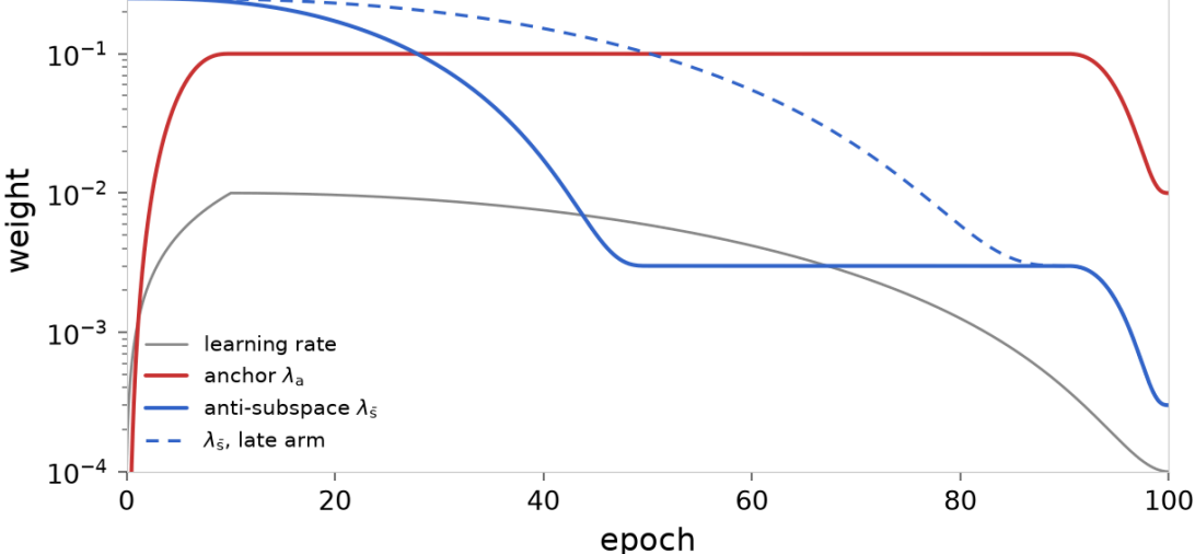
The three schedules at the scoring rung ( \lambda_a = 0.1 ), log scale. The anti-subspace term opens at 2.5\lambda_a dominant before the anchor arrives, and anneals to 0.03\lambda_a by epoch 50 (the M1/ex-2.9.1 keyframes, mapped by fraction of training). The dashed line is the span-anti-late arm, which reaches the hold ratio at epoch 90 instead. From epoch 90 the anchor and anti-subspace weights share the end-of-training anneal to a floor of 0.1\times their held values.
