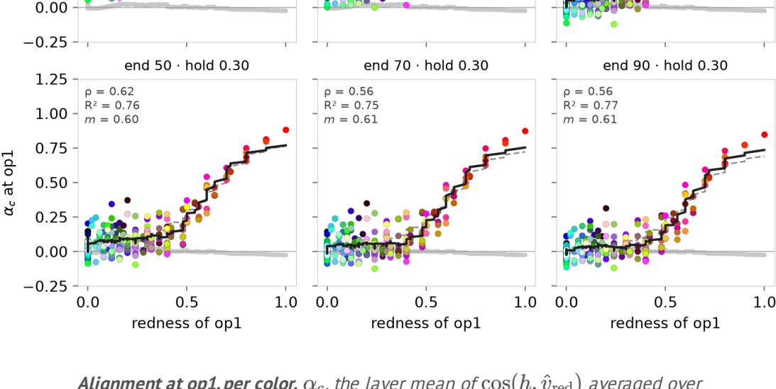
Alignment at op1, per color. \alpha_c , the layer mean of \cos(h, \hat{v}_{red}) averaged over seeds, against the redness of the color. Columns are the anneal endpoint, rows the hold ratio, as in the trajectory figure. One mark per color, drawn in that color; the heavy line is a 25-color sliding mean over the redness ordering, and the flat grey band is the same sliding mean for the un-anchored control. The dashed line is \text{sim}^1 \cdot ^5 rescaled onto the response by least squares – the shape the R^2 track scores against, so the marks' distance from it is what that statistic measures. Per-panel statistics: both grading gates sit at 0.8, and a pure step response can reach at most \rho = 0.75 or R^2 = 0.73 .
