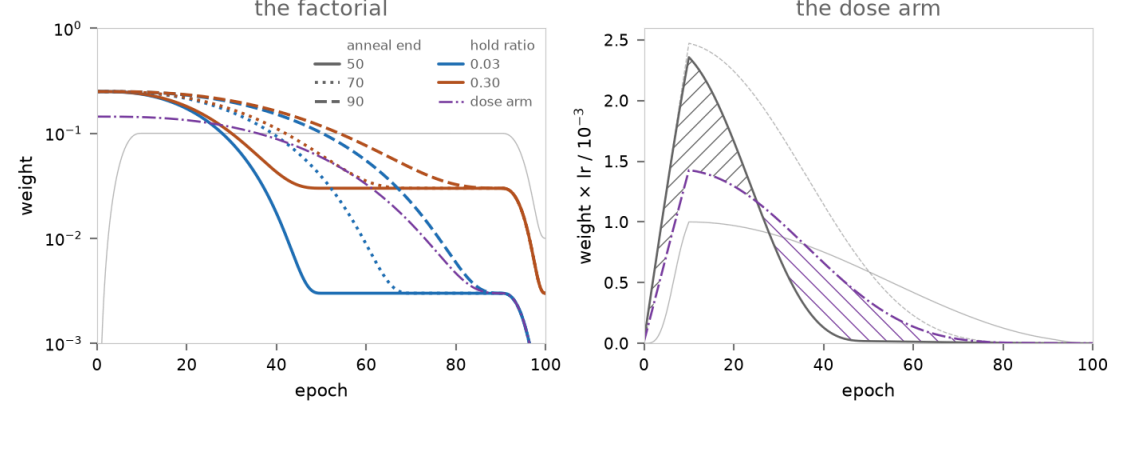
The schedules under test. Left: anti-subspace weight λ s over training, for the six factorial conditions and the dose arm. Right: the dose itself, as its integrand λ s ·lr, so area on the page is repulsion delivered. Hatching shows where the dose arm falls short of the reference early and where it makes that back late. Ghost ink in both panels: the anchor weight λ a ; on the right, also end90-hold03 , the schedule the arm was scaled down from.
