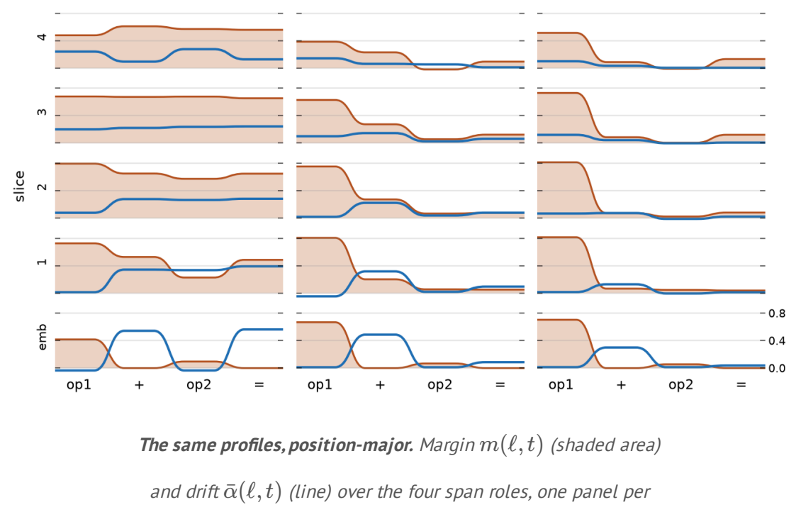
The same profiles, position-major. Margin m(\ell, t) (shaded area) and drift \bar{\alpha}(\ell, t) (line) over the four span roles, one panel per residual slice with the embedding at the bottom — the transpose of the figure above, in the layout the weight profiles under H4 use. Columns: the span mean, the primary, and the op1 oracle.
