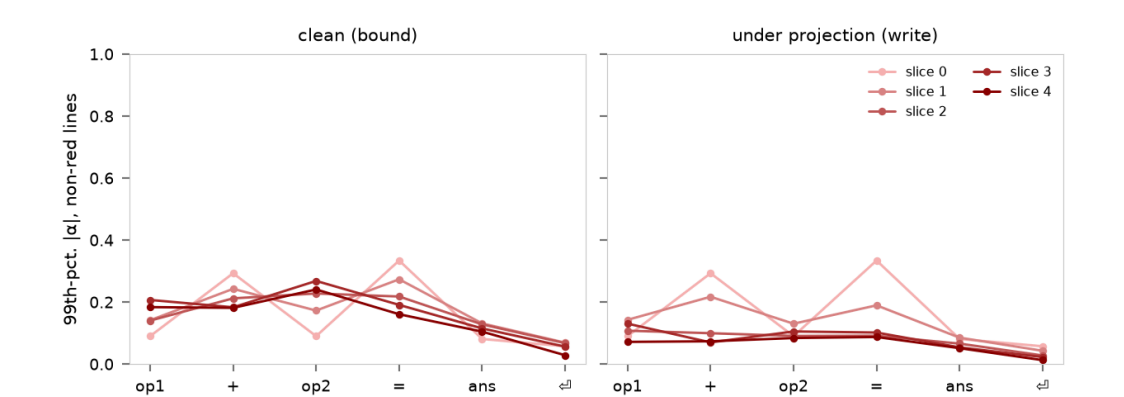
The bound and the write under projection , fallback condition. The 99th-percentile alignment over the non-red lines at each (slice, position), seed mean, on the shared 0–1 scale. Left, the clean map, whose arcsine is the bound; right, the alignment arriving at the operator under projection , whose arcsine is the write. Slices run from the embedding (lightest) to the last block (darkest). A deeper line above its clean value would mean a block re-writes the axis after it was removed upstream, which is what a wider edit looks like.
