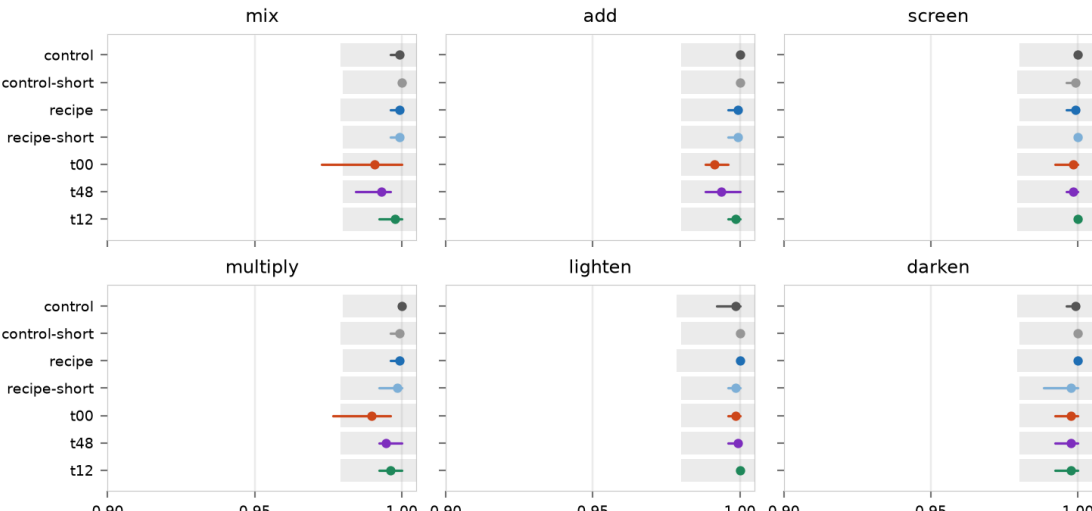
Holdout exact match per op, against the gate. One panel per op; conditions down the side, in their own ink. Each dot is the seed mean, the bar the seed range. The grey strip behind a row is \pm 0.02 around the seed-mean accuracy of the control of the same length, so a dot outside its strip misses the H1 gate; the two control rows carry their own strips for reference.
