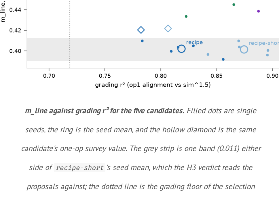
m_line against grading r^2 for the five candidates. Filled dots are single seeds, the ring is the seed mean, and the hollow diamond is the same candidate's one-op survey value. The grey strip is one band (0.011) either side of recipe-short 's seed mean, which the H3 verdict reads the proposals against; the dotted line is the grading floor of the selection rule (0.719, before its 1\sigma margin). The adopted point is labelled ★.
