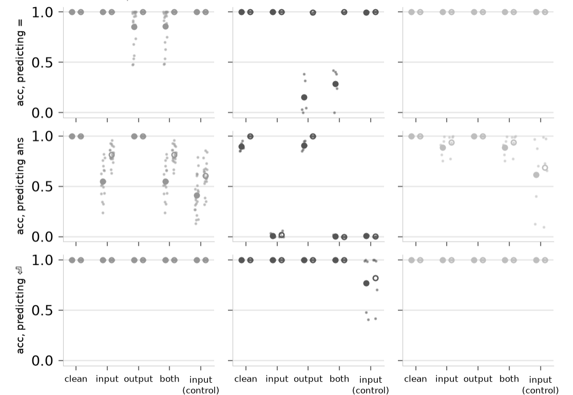
Next-token accuracy on the mix probe lines under each strip, on the stored checkpoints. Rows are the predictions of = , the answer, and the newline; columns are the stored arms. Filled markers are the seed means on the red lines, hollow on the non-red, with one small dot per seed. input strips the axis component from the syntax embeddings and keeps the original table as the readout; output the reverse; both strips it from the shared table; the control moves the embeddings the same distance along a random direction off the axis.
