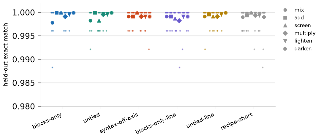
Held-out exact match per op, by arm. One marker shape per op, the seed mean, with one small dot per seed; the y axis starts at 0.98. The reference is ex-2.2.3's production recipe.
