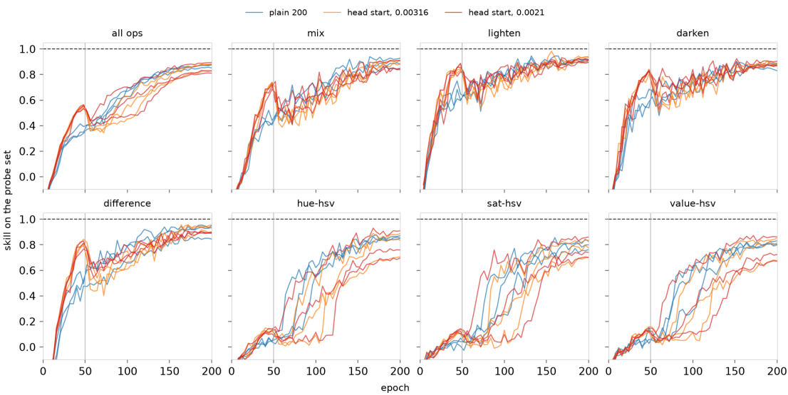
Skill against epoch. Seeds 601–603, one line per run. The vertical line marks the end of the first cycle.
