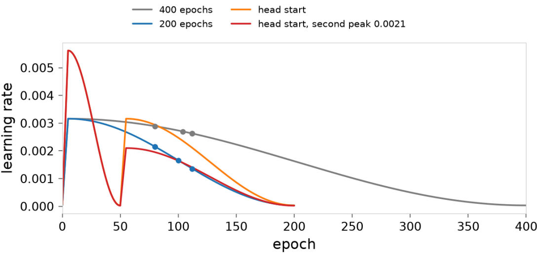
The four schedules. Learning rate against epoch, as the training code computes it. Each dot is the point at which the HSV-channel skill of a plain run of ex-2.2.19 first passed 0.5, one per seed; seeds that passed at the same epoch overlap.
