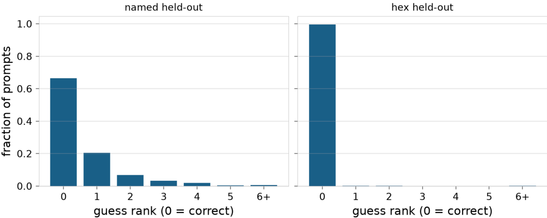
Rank of the emitted answer among the candidate vocabulary of the form, ordered by distance to the true mix; rank 0 is the correct answer. Center condition, pooled over seeds.
