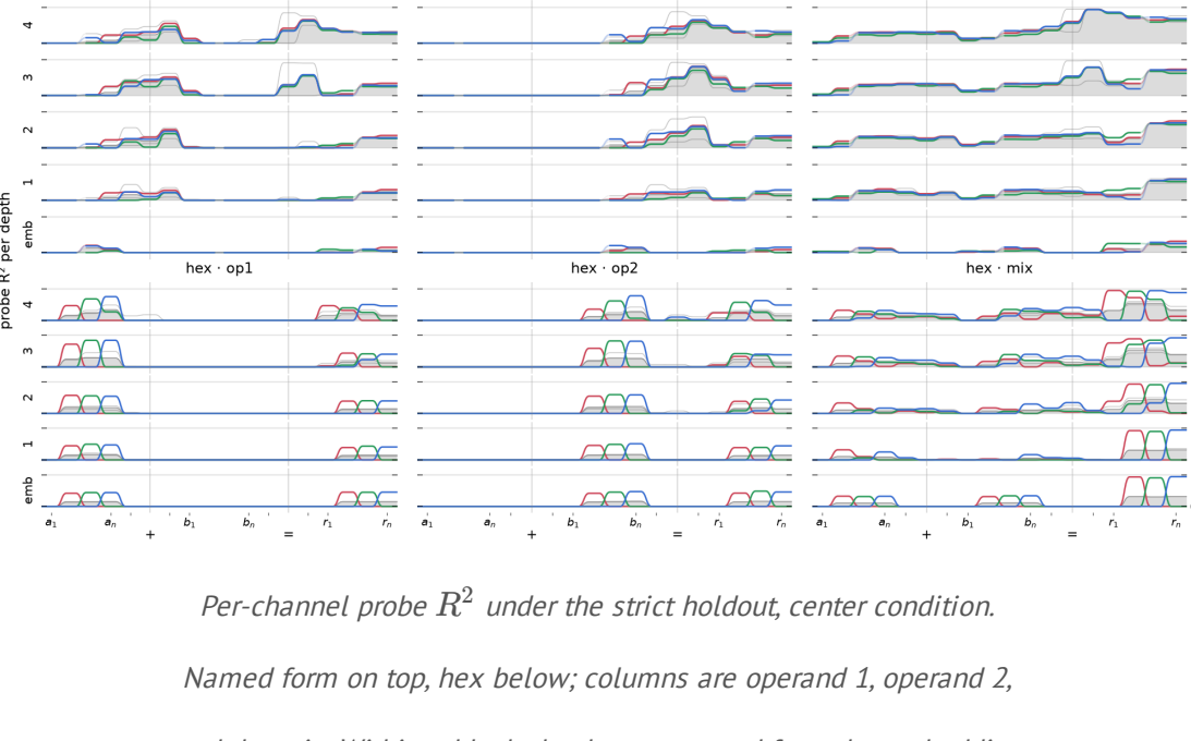
Per-channel probe R^2 under the strict holdout, center condition. Named form on top, hex below; columns are operand 1, operand 2, and the mix. Within a block, depth runs upward from the embedding and the x axis across the grammar landmarks, one step-line per RGB channel. The grey area is the three-channel mean, and the two hairlines are the highest and lowest of the three seeds.
