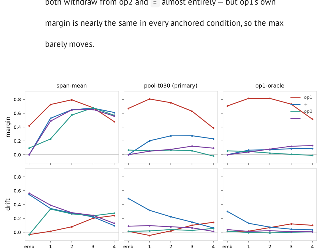
Where the margin and the drift live. Margin (top) and drift (bottom) by span role, per slice, seed means: m(\ell, t) and the unweighted mean alignment \bar{\alpha}(\ell, t) . Columns: the span mean, the primary, and the op1 oracle. The scored statistics take the per-slice max over these lines ( m_{\text{span}} from the top row, \bar{\alpha}_{\text{span}} from the bottom), so a single high line is all either statistic sees.
