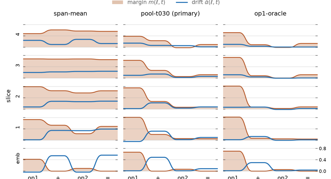
The same profiles, position-major. Margin m(\ell, t) (shaded area) and drift \bar{\alpha}(\ell, t) (line) over the four span roles, one panel per residual slice with the embedding at the bottom – the transpose of the figure above, in the layout the weight profiles under H4 use. Columns: the span mean, the primary, and the op1 oracle.
