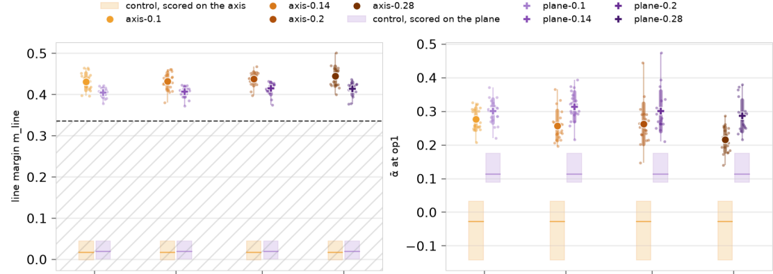
The two quantities the treatment acts on. Left, the line margin, which the anchor term optimizes: the manipulation check, with a heavier pull expected to raise it. Right, \bar{\alpha} at op1, which the anti-subspace term acts on, with no direction attached to it. The tinted box under each column is the un-anchored control's seed range, scored on that column's subspace: on the axis for the axis conditions and on the plane ( control-plane ) for the plane ones. An unsigned two-dimensional alignment sits higher than a signed one-dimensional one for every state, so the two subspaces compare against different boxes.
