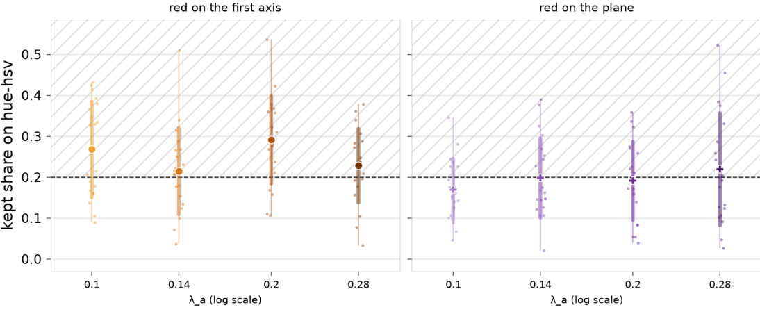
Kept share on the hue-hsv removal lines along the ladder. Left, red on the first axis ; right, red on the plane . Each column is one condition: 20 faint seed dots, a thin bar spanning the seed range, a thick bar spanning one standard deviation either side of the mean, and the seed mean as the large mark. H1 is about the height of the thick bar rather than where the mark sits. The dashed line is the 20% gate, hatched above.
