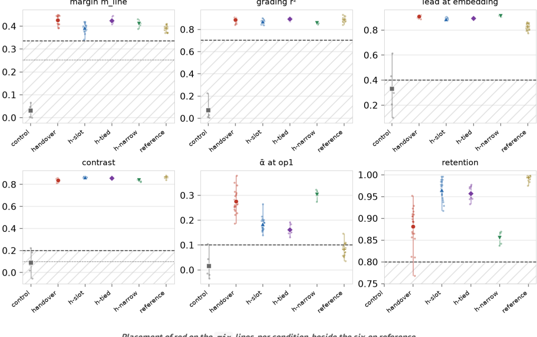
Placement of red on the mix lines, per condition, beside the six-op reference. The read is on mix because the gates were set on mix at ex-2.2.3, so these numbers compare with the reference's. One panel per statistic; each small dot is one seed, the larger mark the seed mean, and the thin bar the seed range, with ex-2.2.3's twenty reference seeds at the right. The dashed line is the gate (margin 0.336, grading r^2 0.704, lead 0.4, contrast 0.2, retention 0.8), the hatched region the side that misses it, and the dotted line the partial level where there is one. The retention column for control is empty because there is no anchor for it to hold. On the \bar{\alpha} panel the dashed line is the 0.1 the earlier experiments gated, which here is a prediction: we expected the untied conditions above it.
