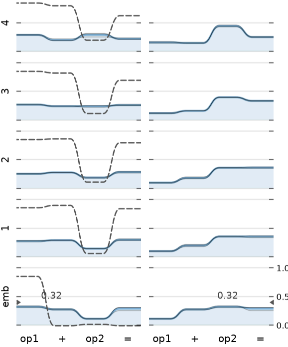
Softer – \tau = 0.5 ; deep-slice op2 contrast +0.17 \pm 0.01 .
