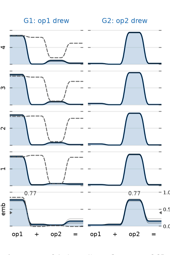
The primary – \tau = 0.1 ; deep-slice op2 contrast +0.85 \pm 0.01 .
