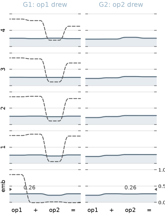
Near the span mean – \tau = 2.5 ; deep-slice op2 contrast +0.03 \pm 0.00 .
