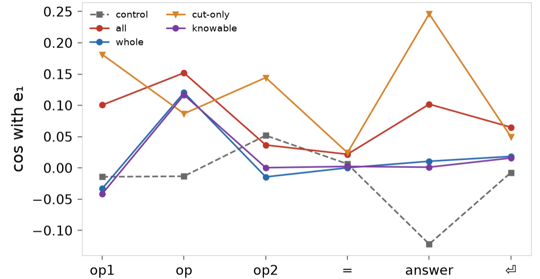
Each role on whole lines (post hoc; planned, no gate). The seed-mean cosine with e1 at the last block at each role, over every op's probe lines, which are whole lines.
