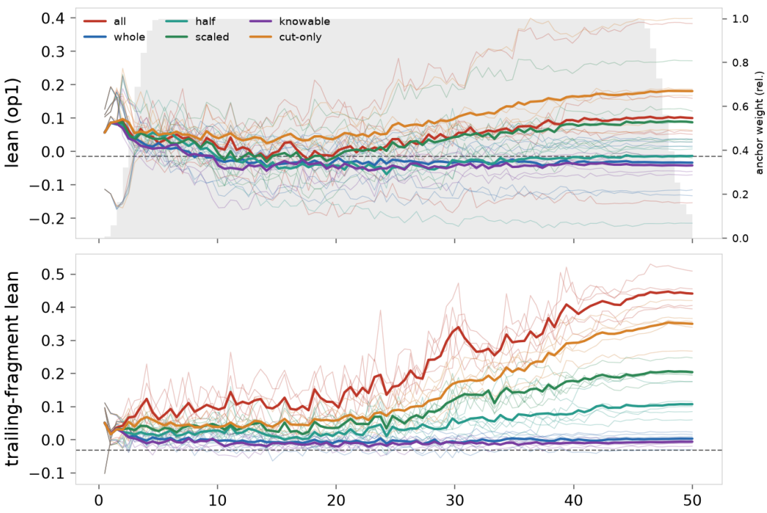
The lean through training. Top: the lean at the last block on the trajectory probe lines, recorded every 50 steps; the thick line is the seed mean and the hairlines are the seeds. The grey silhouette is the anchor weight's schedule (right-hand scale, relative to its peak). Bottom: the trailing-fragment lean (H3), pooled over ops. The dashed lines are the control's values at the end of training; the control records no trajectory.
