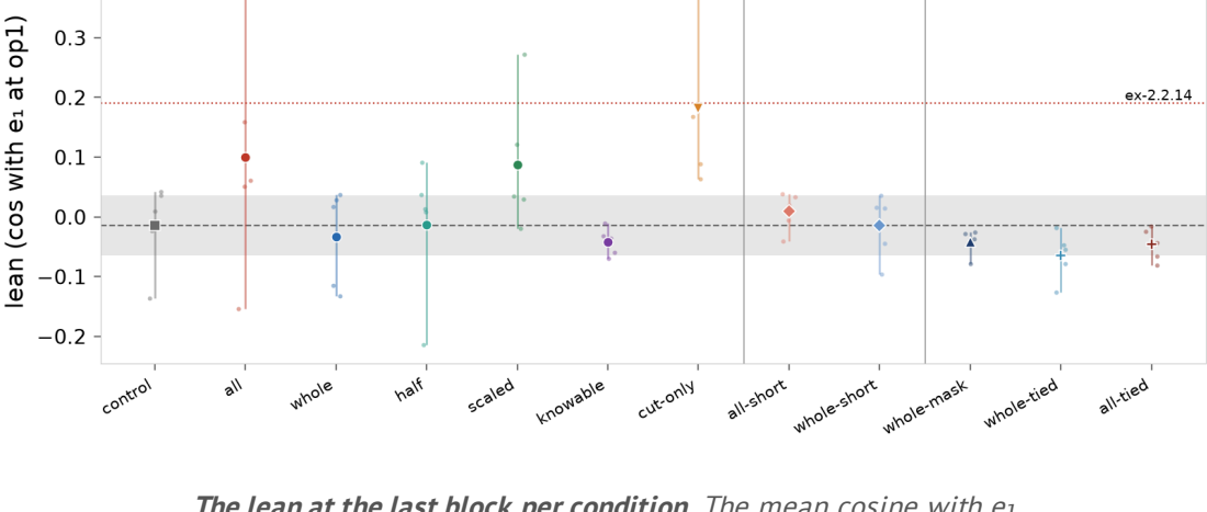
The lean at the last block, per condition. The mean cosine with e_1 at the first operand, over every op's probe lines, one small dot per seed and the seed mean as the large mark. The grey band is the control's seed mean \pm 0.05 , the band whole has to land in for H1 to pass; the dotted line is the primary of ex-2.2.14 (0.19). The groups are the policies, the halved windows, and the model arms.
