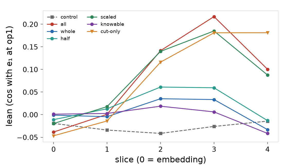
The lean at each slice. The seed mean of the cosine with e_1 at the first operand, over every op's probe lines, from the embedding (slice 0) to the last block, for the control and each policy.
