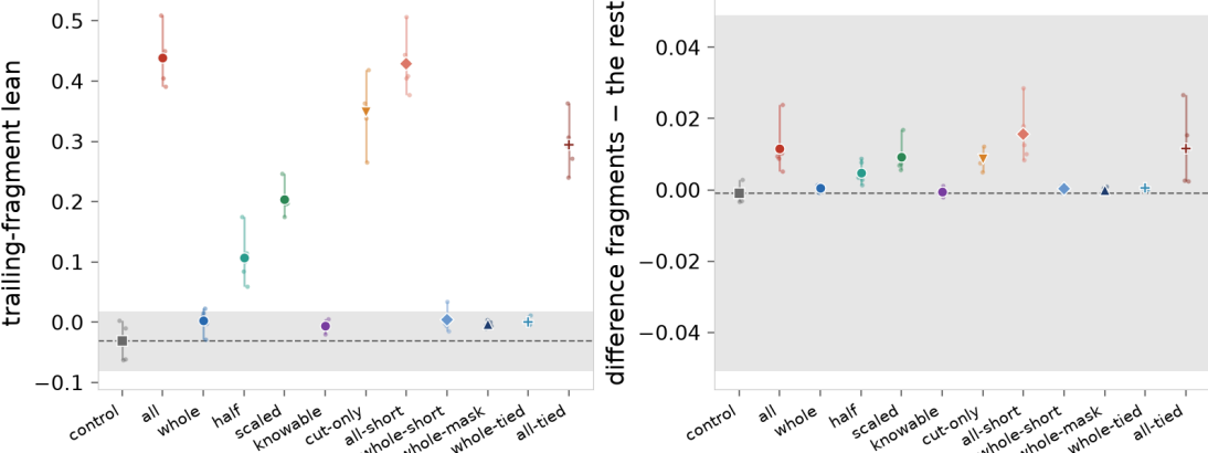
Trailing fragments at the last block. Left: the mean cosine with e1 over every position of every trailing fragment of every op.
