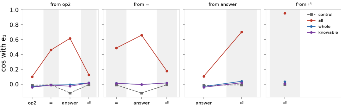
Where a trailing fragment leans. The seed-mean cosine with e1 at the last block at each position of a trailing fragment, pooled over ops, one panel per role the fragment starts at. The shaded columns are the syntax tokens = and ↵ , which carry no color.
