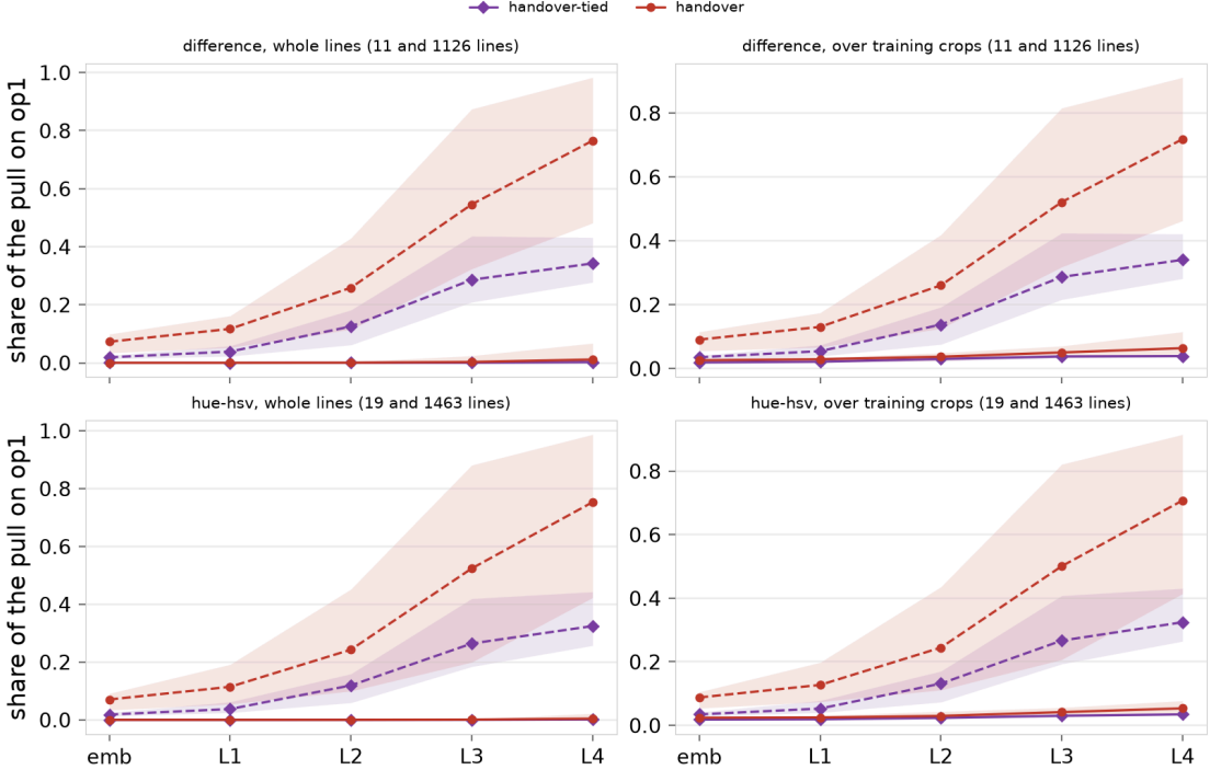
The share of the pull that lands on op1, on lines that can earn a label only through their answer. Probe lines with both operands non-red, split by a red answer (solid) or a non-red one (dashed), on the two conditions with the whole-line labeller. Top row difference , bottom row hue-hsv ; the line counts are in the panel titles. Left: the softmax weight the anchor term assigns op1 on the whole line. Right: the same weight averaged over the ways a training crop shows the line, where a crop that cuts the line before the answer leaves the pull to the prompt. The shares are read from the final checkpoint; the unlabelled lines receive no pull, so theirs is the share the term would assign if they did. Lines are seed means and bands the seed range.
