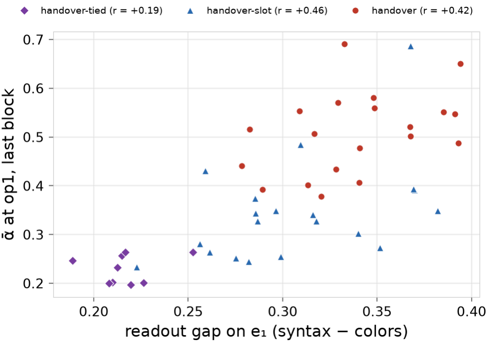
The readout gap against \tilde{\alpha} at op1, per seed. Each mark is one run: on the x axis the syntax words' mean e_1 in the readout table less the colors; and on the y axis \tilde{\alpha} at op1 at the last block. The legend gives the Pearson r within each condition.
