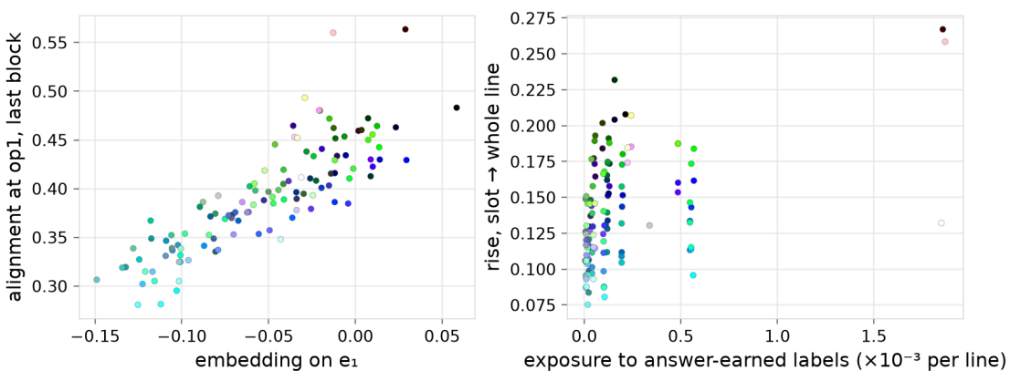
What predicts the lean of a non-red color, on handover . Left: the embedding of the color on e_1 against its last-block alignment at op1 ( r = +0.84 ). Right: the exposure of the color to labels earned through the answer (its per-line probability as op1, mean over the eleven ops and every partner) against the rise in its lean from handover-slot to handover ( r = +0.42 ; the rise has a spread of 0.04 over colors). Non-red colors only, seed means.
