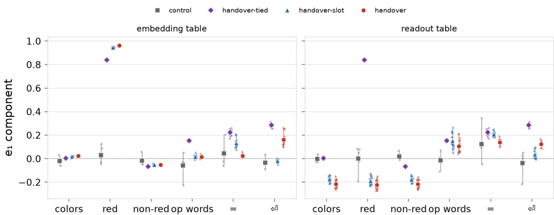
The e_1 component of the tables, by token group. Left: the embedding table.
