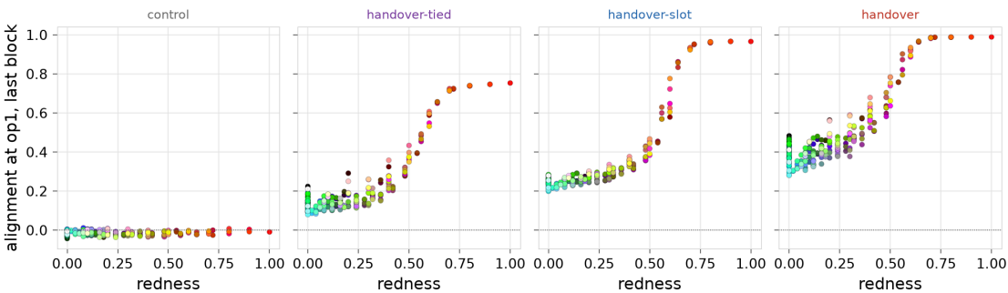
The alignment of each color at op1 against its redness, at the last block. One mark per grid color in the color itself, the seed mean per condition. Redness is r(1 - g/2 - b/2) on the unit cube, the grading target.
