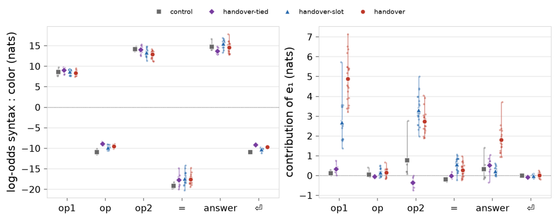
The next-token log-odds and the part e_1 contributes, by position, at the last block. Left: \log P(\text{syntax word next}) - \log P(\text{color next}) , mean over the mix probe lines. Right: the change in that log-odds when the part of every logit that comes from the e_1 coordinate is removed, so a positive value means e_1 argued for a syntax word.
