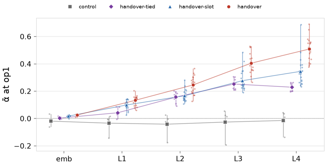
\bar{\alpha} at op1 per slice. Each column is the seeds of one condition at one slice: the mean over the 216 grid colors of the cosine between the state of the color at the first operand and e_1 , on the mix probe lines. The lines join the seed means.
