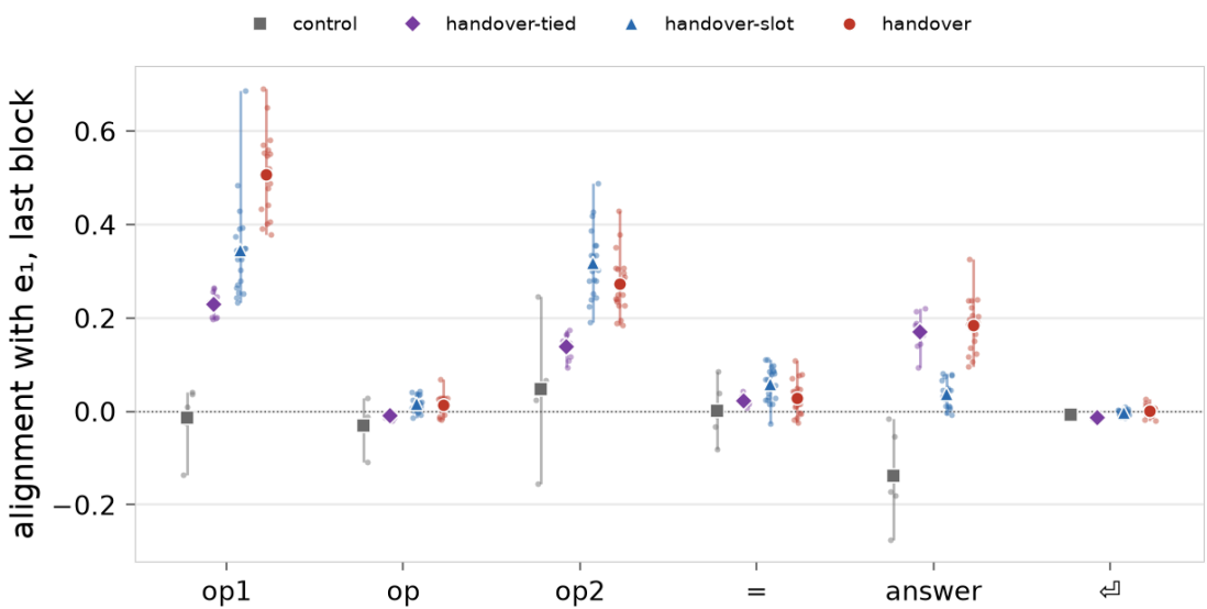
Alignment with e_1 by position, at the last block. The mean over mix 's probe lines of the cosine between the state at each position and e_1 . The positions alternate between predicting a syntax word (op1, op2, answer) and predicting a color (op, =, ⇐).
