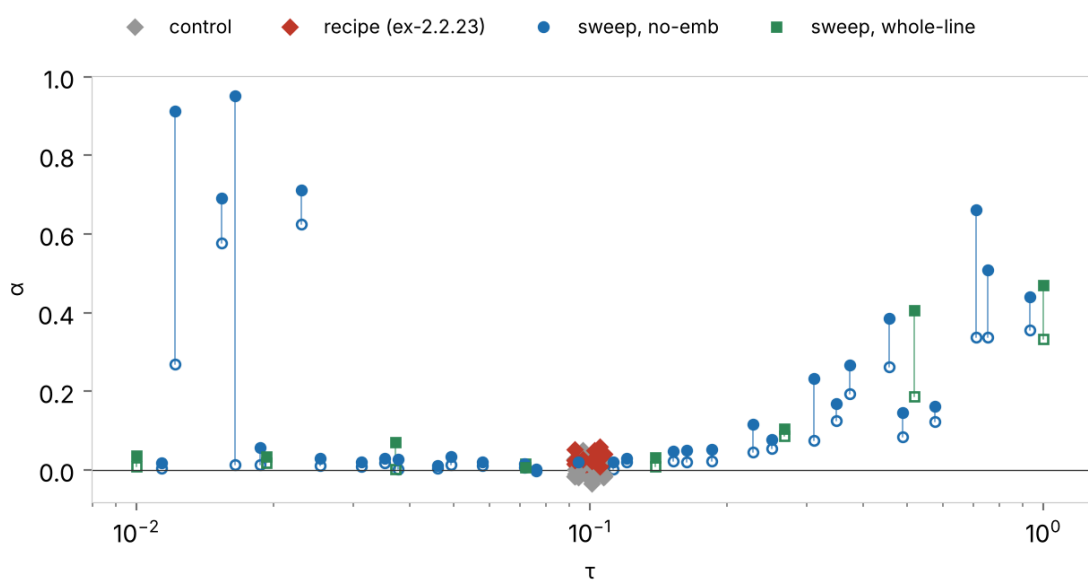
How much anchor the = tokens hold, by pool temperature. On the held-out difference contexts, \alpha at the first = (open marks, where no example has been shown) and at the query = (filled marks, after three), joined per run. Circles: the no-emb arm of the sweep; squares: its whole-line arm; diamonds: the 400-epoch anchored runs of ex-2.2.23, at the recipe \tau , spread sideways so they can be told apart; grey: the controls of ex-2.2.23, drawn at the same \tau .
