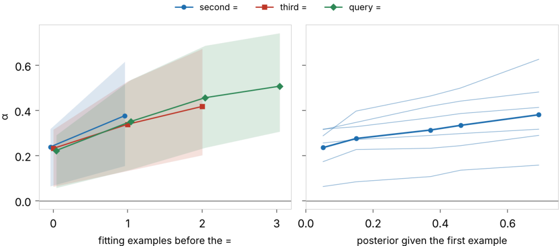
What \alpha at the = follows, on the six rising trials. Left: \alpha against the number of examples before the = that fit difference, one line per = index (the second and third example and the query), the mean over trials with the range as a band. Right: \alpha at the second = against the posterior given the first example alone, in bins; the first bin holds the examples that do not fit, and the rest split the fitting examples by how specific they are. One thin line per trial, the mean in bold. A bin with fewer than 20 contexts is left out.
