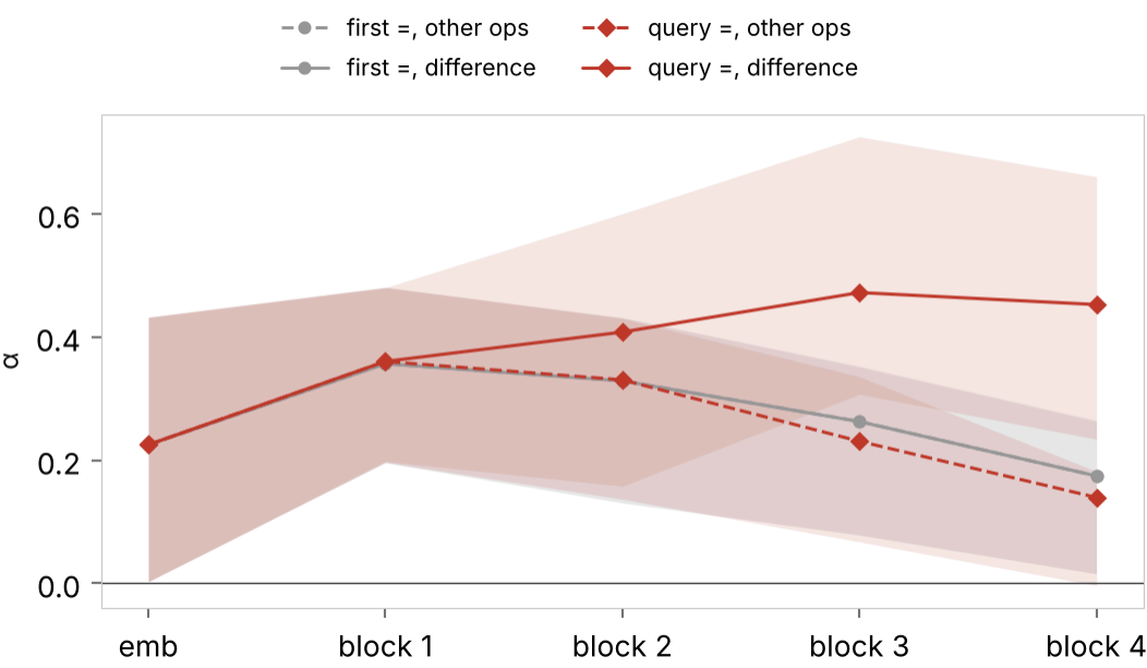
Where the anchor at the = sits by depth, on the six rising trials. \alpha at the first = and at the query = , on difference contexts and on the other ops' contexts, at each slice from the embedding (emb) to the output of block 4. The mean over trials, with the range as a band.
