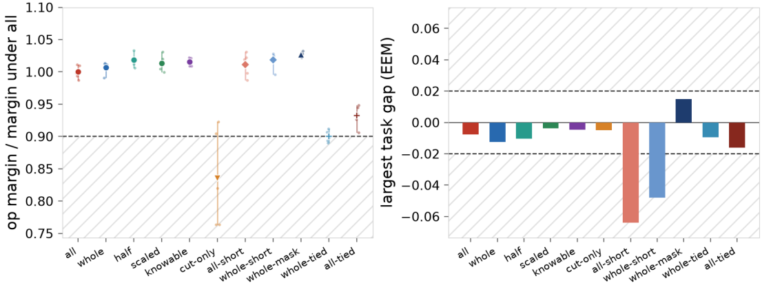
The anchor and the task, per arm. Left: the op margin as a share of the seed-mean margin under all , one small dot per seed and the seed mean as the large mark; H2 asks for at least 90% (dashed; hatched below). Right: the gap in held-out expected exact match from the control, for the op furthest from it; H2 asks for at most 0.02 either way (dashed; hatched beyond).
