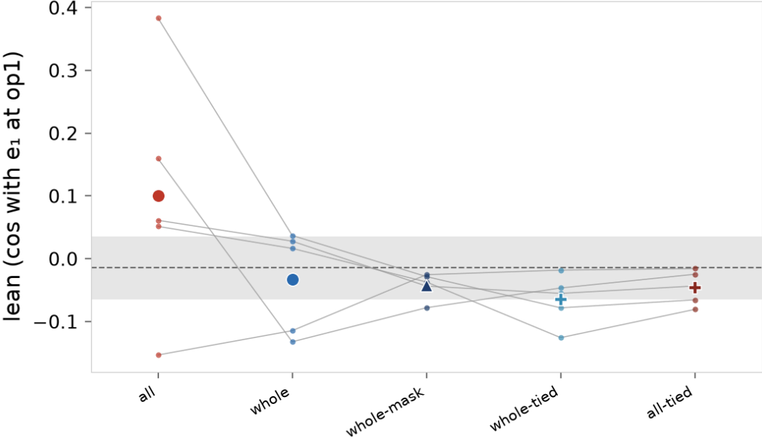
The lean under the model arms, by seed. The lean at the last block, one dot per seed and the seed mean as the large mark. The thin grey lines join the dots of one seed, which trains on the same windows and labels in every column. The grey band is the control's seed mean ± 0.05.
