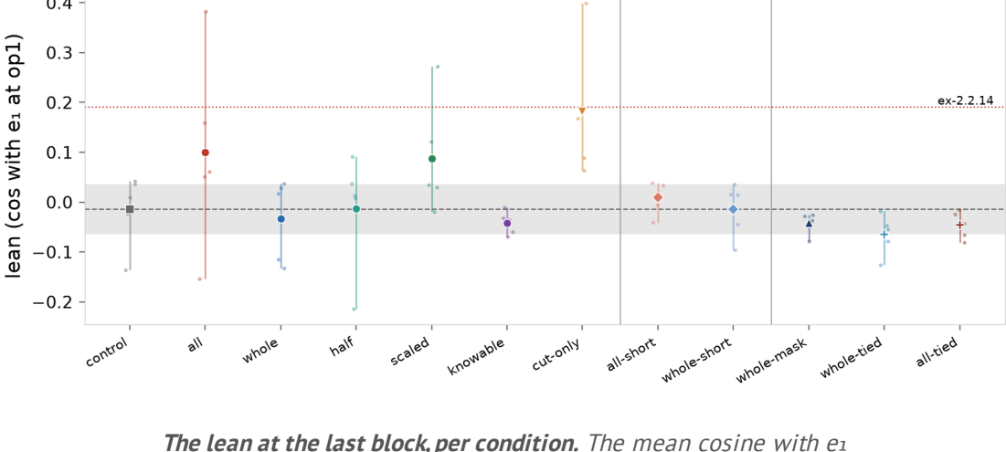
The lean at the last block, per condition. The mean cosine with e_1 at the first operand, over every op's probe lines, one small dot per seed and the seed mean as the large mark. The grey band is the control's seed mean \pm 0.05 , the band whole has to land in for H1 to pass; the dotted line is the primary of ex-2.2.14 (0.19). The groups are the policies, the halved windows, and the model arms.
