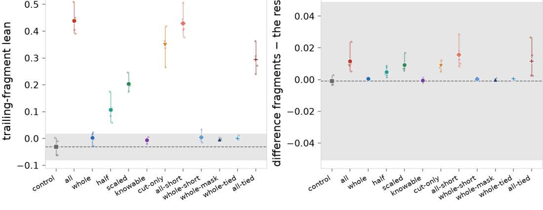
Trailing fragments at the last block. Left: the mean cosine with e1 over every position of every trailing fragment of every op. Right: the same over the difference fragments less the mean over the rest. One small dot per seed, the seed mean as the large mark; the grey band is the control's seed mean \pm 0.05, for scale.
