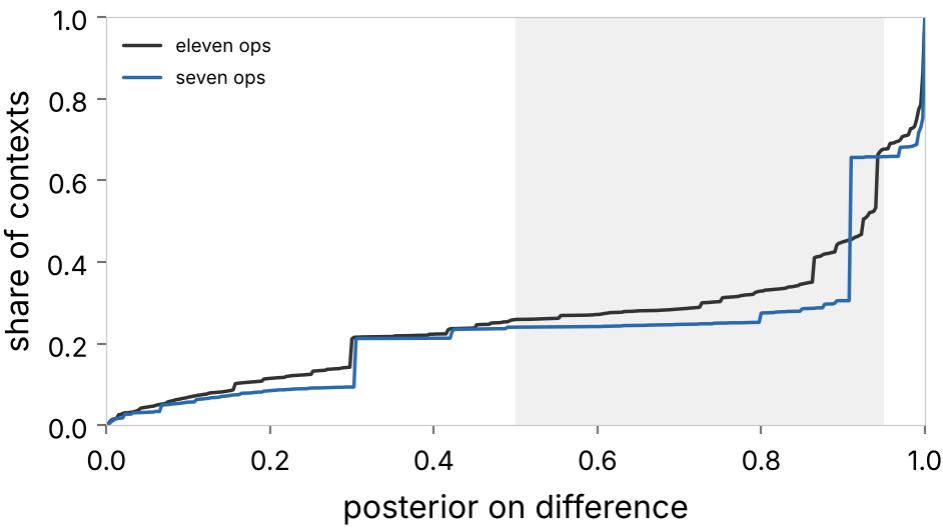
The stimulus on the seven-op table. The share of difference contexts whose posterior on difference is at most the value on the x -axis, at three examples, \rho = 0.3 , and cube noise at \kappa = 0.02 . The shaded band is the middle band. 20,000 sampled contexts per curve.
