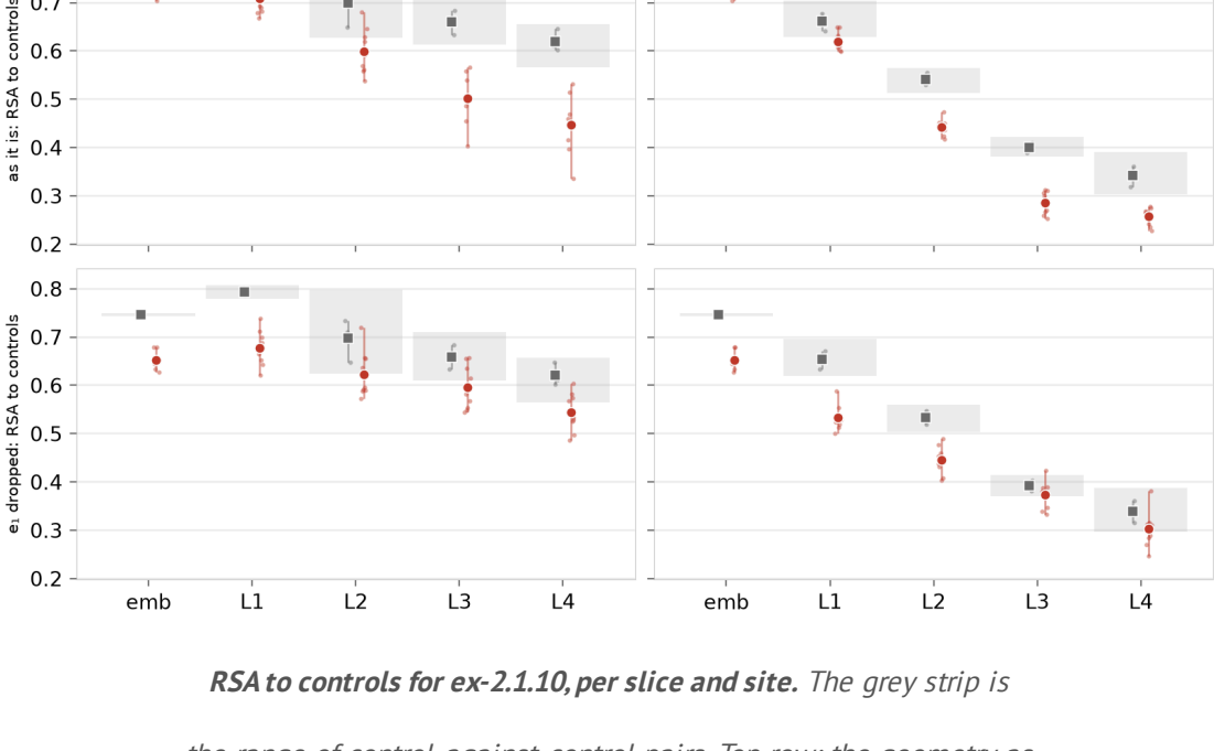
RSA to controls for ex-2.1.10, per slice and site. The grey strip is the range of control-against-control pairs. Top row: the geometry as it is. Bottom row: the anchor axis e_1 dropped from every run first.
