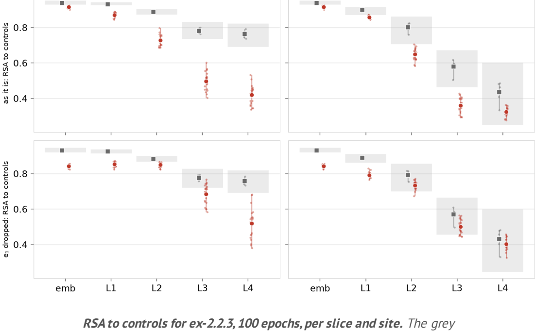
RSA to controls for ex-2.2.3, 100 epochs, per slice and site. The grey strip is the range of control-against-control pairs. Top row: the geometry as it is. Bottom row: the anchor axis e_1 dropped from every run first.
