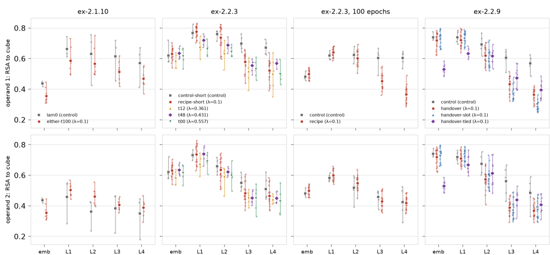
RSA between each run's colour geometry and the RGB cube itself, per slice and site. The cube's distances are the Euclidean distances between the 216 grid colours in RGB. Each dot is one seed, the larger mark the seed mean. A run that arranges the colours as the cube does scores 1.
