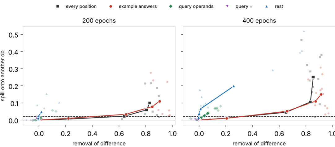
Spill against removal, for each set of positions. One line per set through the doses 0.25, 0.5, 0.75, 1, the seed mean over the runs the rule keeps; the faint marks are those runs at full dose. Both measurements are net of the control at the same seed and length. Dashed: the selectivity criterion of ex-2.2.21.
