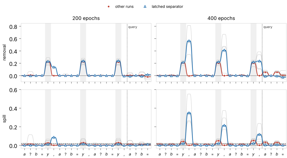
Removal and spill for each position edited alone, at full dose. Top: removal of difference ; bottom: spill onto another op; both net of the control at the same seed and length. The markers are the seed means, over the runs whose separator embedding lies on e_1 (hollow, E3) and over the other runs; the faint lines are single runs. The shading marks the example answers; dashed: the selectivity criterion of ex-2.2.21.
