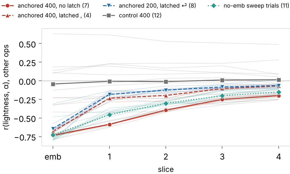
The lightness correlation by slice. Each line is the seed mean of the correlation between lightness and \alpha at the color positions of other ops, with the individual runs as faint lines behind. Circles: 400-epoch runs with no latch. Up-triangles: latched on , . Down-triangles: 200-epoch runs latched on \leftrightarrow . Squares: the controls. Diamonds: the no-emb trials of the \tau \times \lambda_a sweep, \tau from 0.05 to 0.3.
