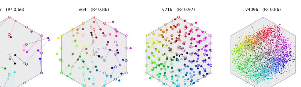
The same embedding tables (seed 0), now read through the probe instead of through variance: each token is placed at the RGB the probe predicts for it, and drawn in the color it actually names. Open rings mark where a token should sit, so the displacement (lines) show the error. R² is the same fit as a single number, averaged over seeds. Rings are left off at v4096, where 4096 of them would bury the colors.
