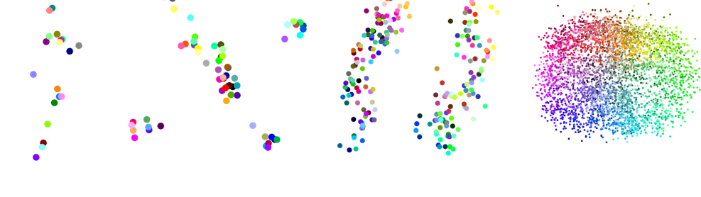
The embedding table, projected onto its own first two principal components (seed 0), with each token drawn in the color it names. Only v4096 shows the hue wheel we thought we might find. The percentage is how much of the table variance its leading three components hold – the most any three directions could – of which the panel draws the leading two.
