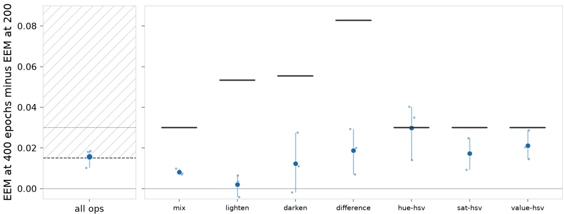
Shortfall of the 200-epoch run from the 400-epoch run, by model seed. The larger dot is the seed mean and the thin bar spans the seeds. Left: all ops, against the gate (dashed) and the end of the partial band (dotted); the hatched side misses. Right: each op, against its tolerance (horizontal bar).
