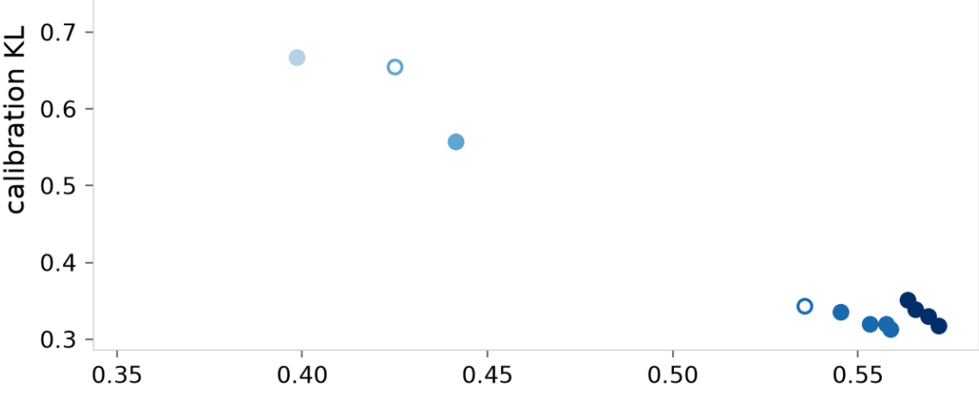
Calibration KL against held-out EEM. One dot per run, one color per length, darker for longer. A filled dot is a run at the rate taken at its length; a hollow dot is a scout run at the other rate.
