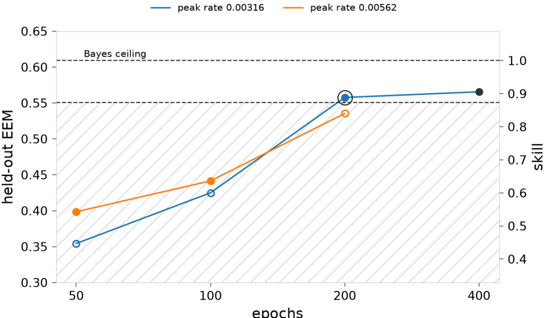
Held-out EEM by length at the scout seed. One line per peak rate. Only the recipe rate was trained for 400 epochs, in ex-2.2.18. Filled dots mark the rate the rule takes at each length. The dashed line is the Bayes ceiling (skill on the right axis), and the hatched region is more than 0.015 below the 400-epoch run. The pick is ringed.
