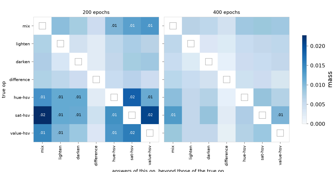
Where the mass goes, by op, at 200 and 400 epochs. Mean over the three fresh seeds, on confident held-out contexts. Rows are the true op. Each off-diagonal square is the mass the model puts on colors the column op can give and the true op cannot, with values of 0.01 and above printed. The diagonal is outlined and left blank. Columns are the seven ops of the set.
