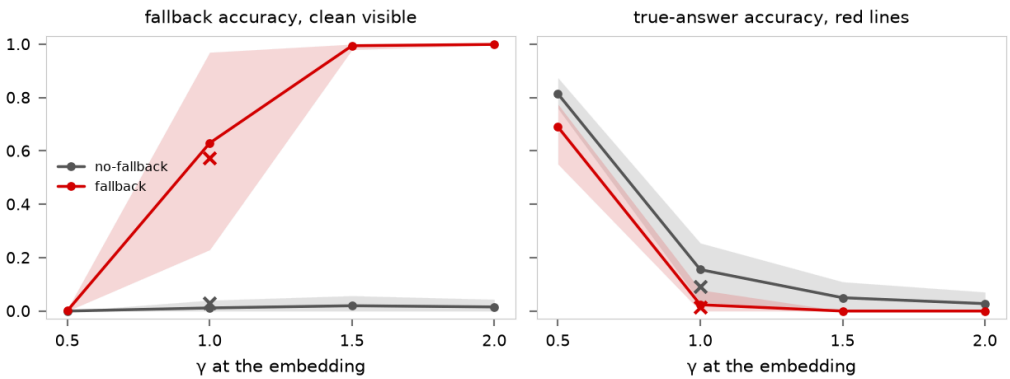
The transfer sweep. Seed mean with the seed range as a band, for the projection operator at the embedding at strength \gamma , every position. Left, fallback accuracy on the red lines with a clean visible operand; right, true-answer accuracy on all red lines. \gamma = 2 is redirect ; \gamma = 1 is the embedding arm of ex-2.2.1. The crosses at \gamma = 1 are the projection row of each condition, which removes the axis at every slice rather than at the embedding alone.
