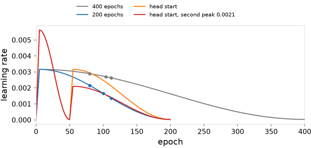
The four schedules. Learning rate against epoch. Each dot is the point at which the HSV skill of a plain run of ex-2.2.19 first passed 0.5.
