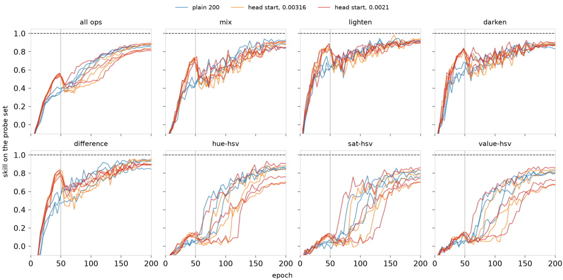
Skill trajectories. Seeds 601–603, one line per run. The vertical line marks the end of the first cycle.
