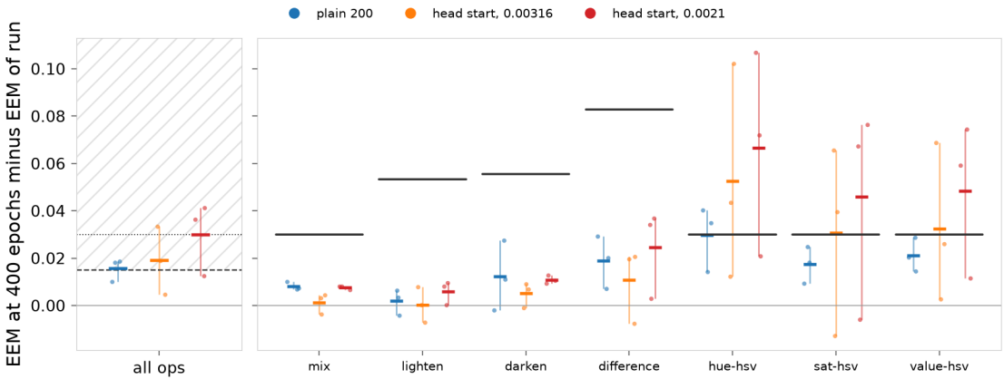
Shortfall from the 400-epoch runs. Seeds 601–603; a dash marks the seed mean. Left: all ops, with the gate (dashed) and the edge of the partial band (dotted). Right: by op, with the tolerance of each op (black bar).
