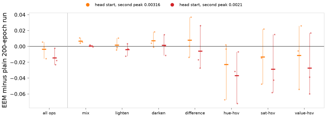
Gain over the plain 200-epoch run. Seeds 601–603; a dash marks the seed mean. Above the line, the head start scored higher.
