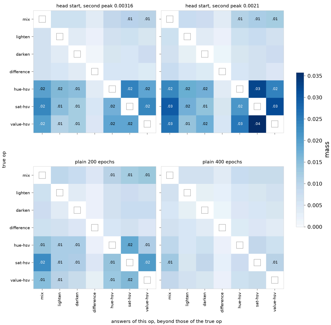
Op confusion , mean over seeds 601–603, on confident contexts. Each square is the mass on the answers of the column op that the true op cannot give; values of 0.01 and above are printed.
