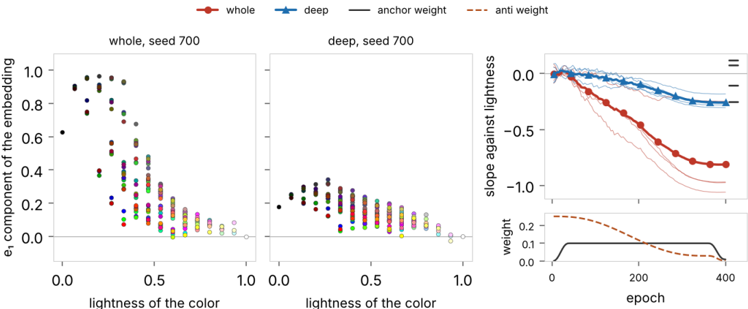
The lean of the color embedding table. Left and middle: the e_1 component of each of the 216 color embeddings against its lightness at the end of training, one run of each arm, each dot drawn in its own color. Right: the slope of that component against lightness along training, one hairline per run and the seed mean bold; the ticks at the right edge are the controls at the same seeds. deep-clean is zero throughout and not drawn. The strip below is the weight of each term, the same in both arms: the anchor weight solid and the anti-subspace weight dashed.
