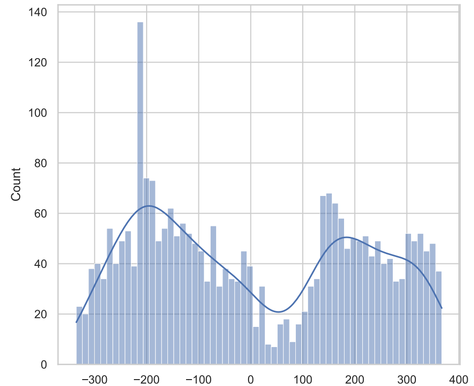
density error
